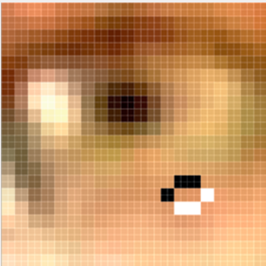
Pixel repetition
